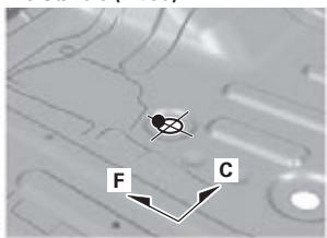
H4, h4 Floor Rear Extension A Locating Hole \varnothing 20 (0.79)
