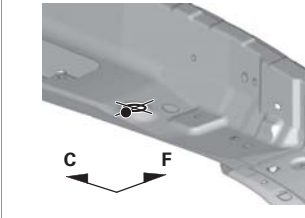
I4, i4 Rear Roof Trim Clip Mounting Hole \varnothing 8.5 (0.335)
