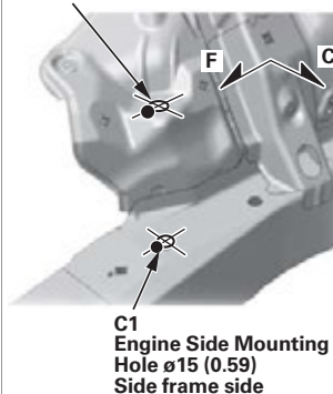
C2 Engine Side Mounting Hole \varnothing 13 (0.51) Wheelhouse side
