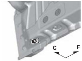
L, l Front Inside Sill B Locating Hole \varnothing 20 (0.79) rear
