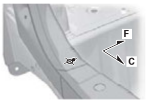
J4, j4 Rear Trim Panel Clip Mounting Hole \varnothing 8.5 (0.335)
