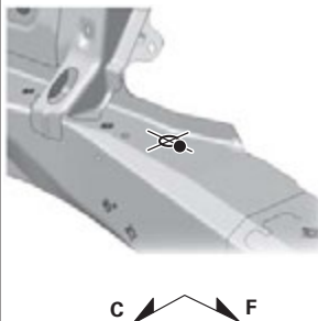
C3 Battery Set Base Mounting Hole \varnothing 9 (0.35)
