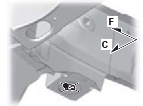
F, f Left Floor Front Extension Locating Hole \phi 32 (1.26) Right Floor Front Frame Locating Hole \phi 32 (1.26)
