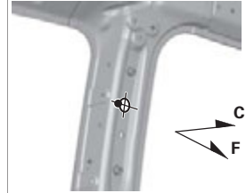
I3, i3 Quarter Inner Upper Pillar Locating Hole \varnothing 13 (0.51)
