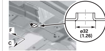
F, f Left Floor Front Extension Locating Hole \phi 32 (1.26) Right Floor Front Frame Locating Hole \phi 32 (1.26)
