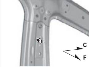
I2, i2 Center Inner Pillar Locating Hole \varnothing 13 (0.51)
