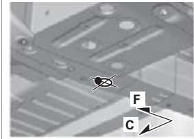
E, e Front Side Frame Gusset Locating Hole \phi 28 (1.10)
