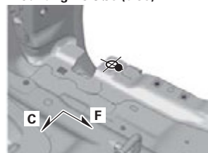
H3, h3 CESS Articulated Harness Mounting Hole \varnothing 9 (0.35)
